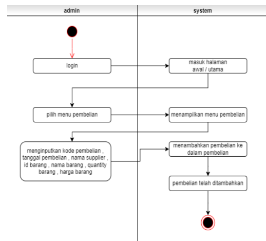
Gambar 3. 11 Activity Diagram Masuk Barang
