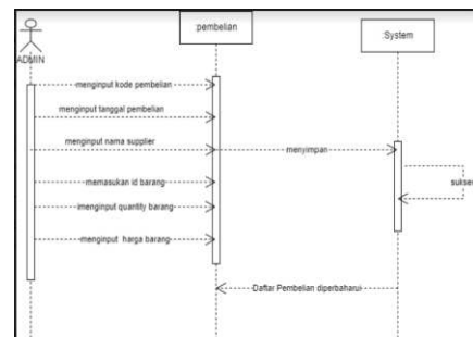
Gambar 3.15 Diagram Sequence Masuk Barang
