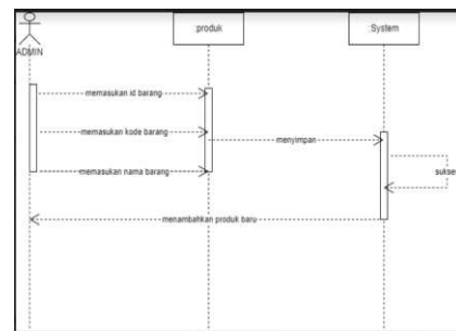
Gambar 3.14 Diagram Sequence Produk
