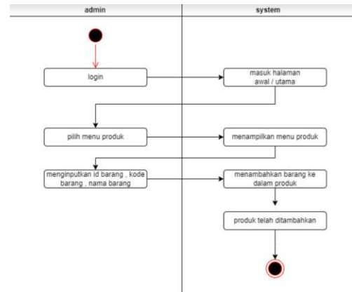
Gambar 3. 10 Activity Diagram Produk
