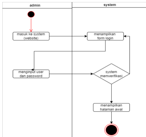
Gambar 3. 9 Activity Diagram Login
