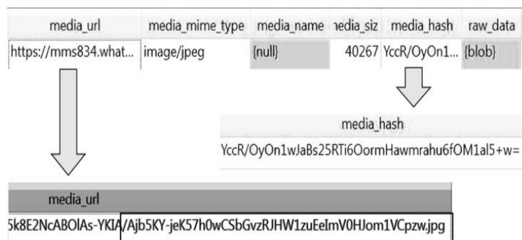
Gambar 7. Multimedia file exchange: recipient side (Anglano, 2014)
