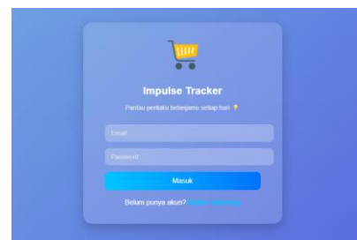
Figure 4. Login Process
