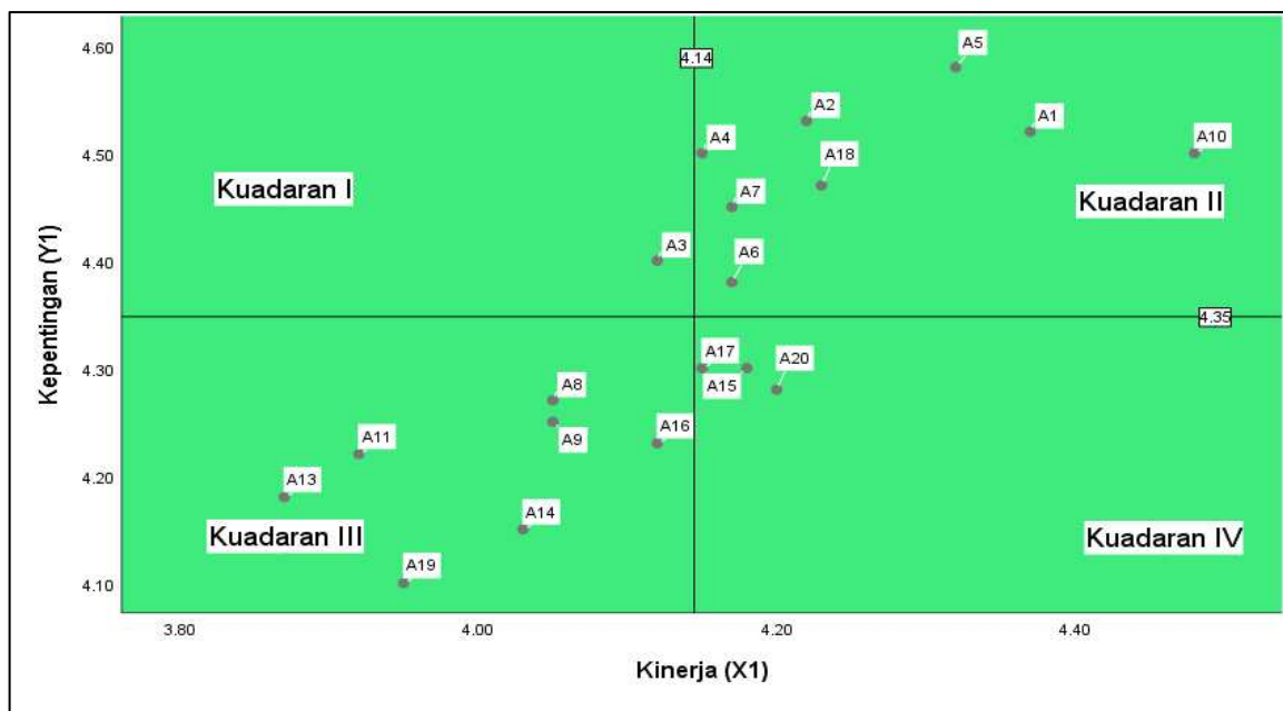
Gambar 4. Diagram Kartesius.
