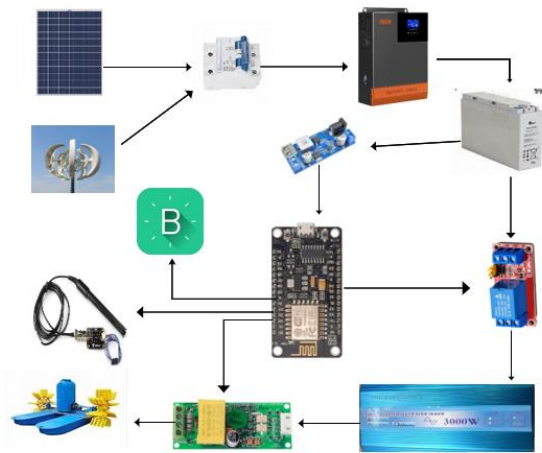
Gambar 2. Desain Hardware
