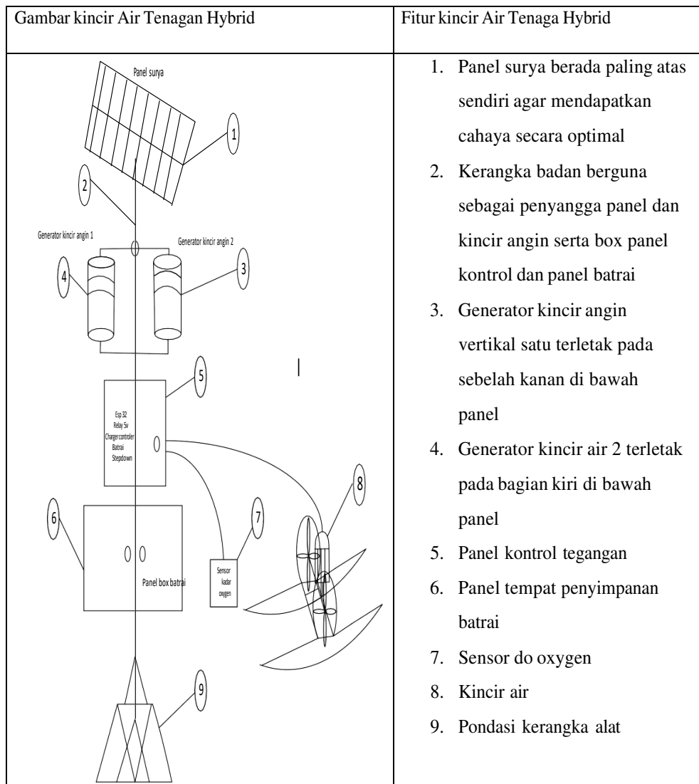
Gambar 4. Desain Prototype
