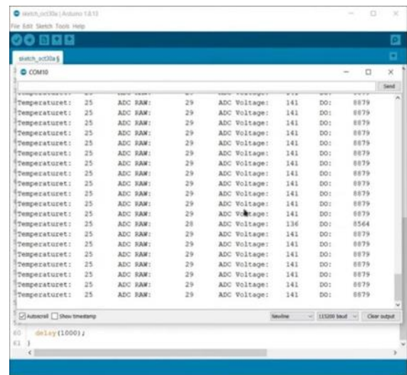
Gambar 6. Uji Kalibrasi Sensor Oxygen
