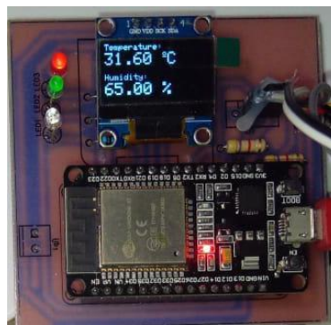
Gambar 4 Node Sensor
