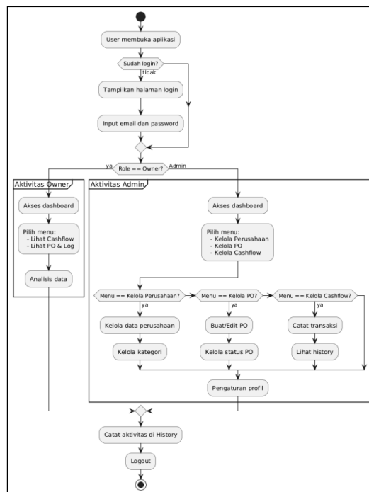
Gambar 3. Activity Diagram
