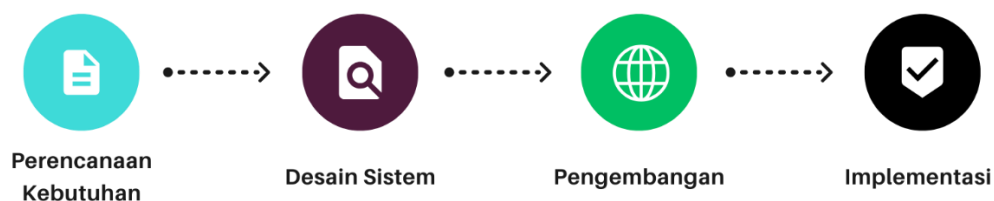
Gambar 1. Alur Penelitian
