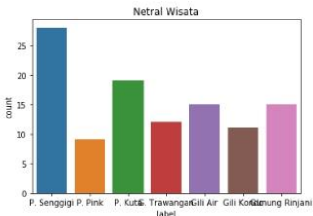
Gambar 9. Sentiment Netral
