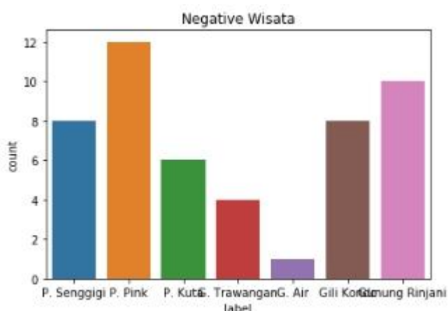
Gambar 10. Sentiment Negative
