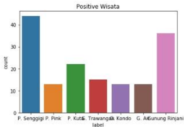
Gambar 11. Sentiment Positive
