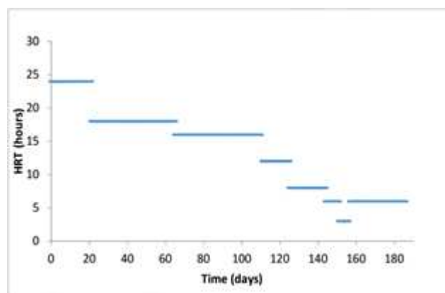
Figure 3. Time course of HRT during reactor operation
