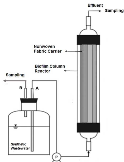
Figure 1. Schematic research equipment of biofilm column reactor
