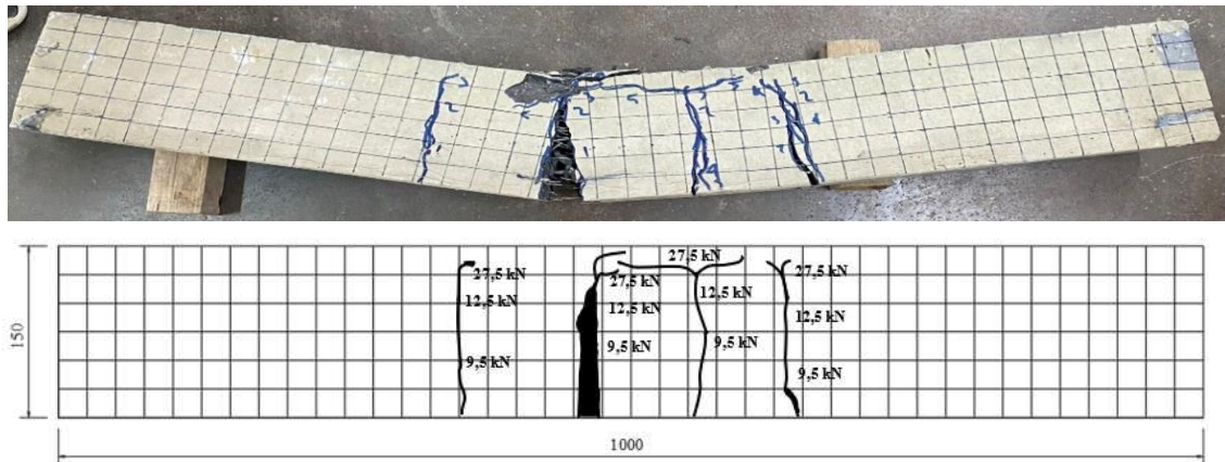
Fig. 14. The crack pattern behavior of PFRSCC beam
