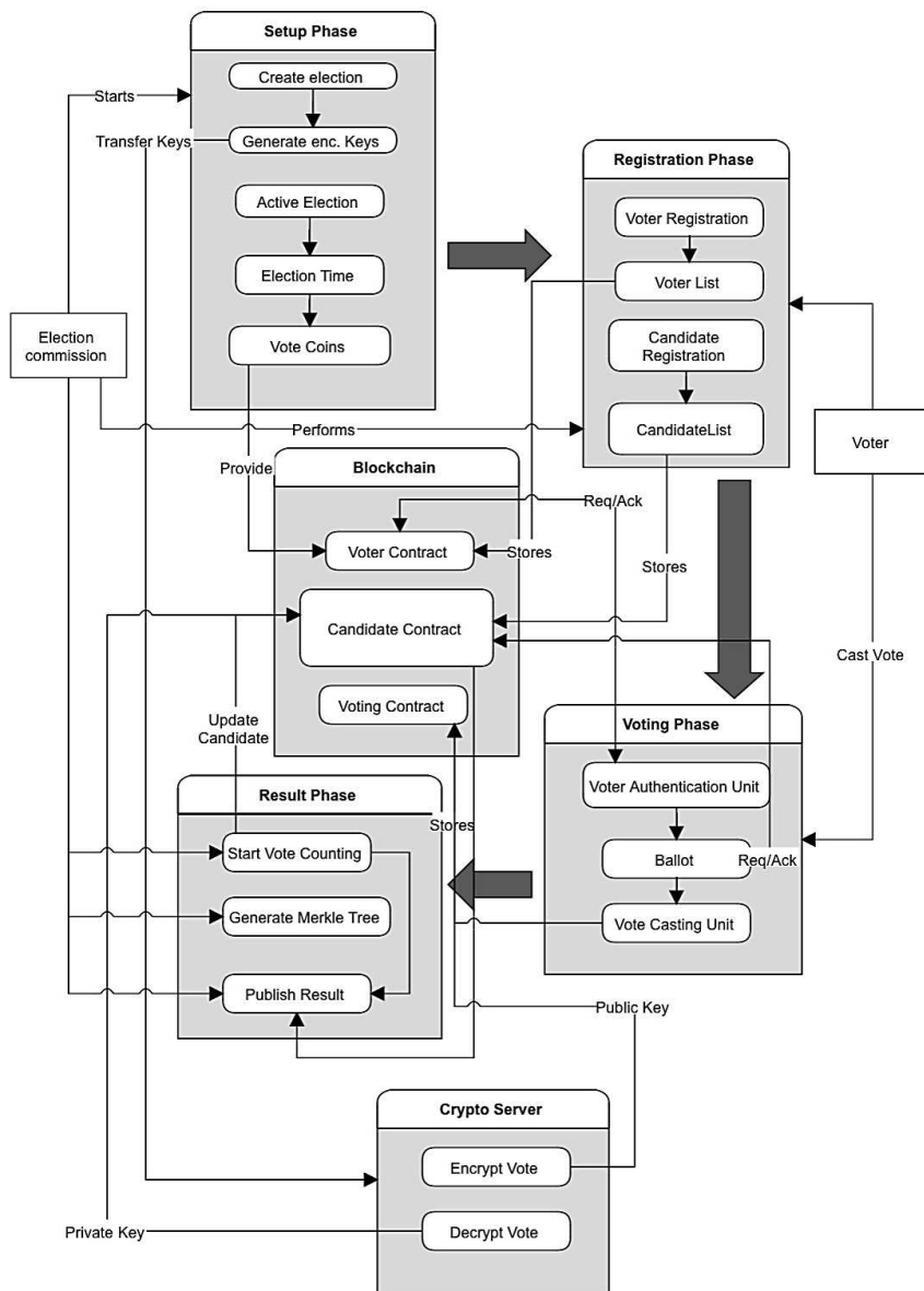
Figure 1. Blockchain based Voting Flowchart
