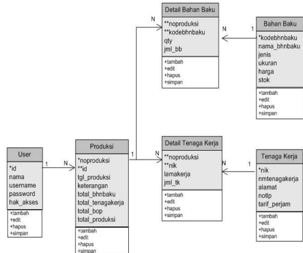
Gambar 2. Rancangan Class Diagram
