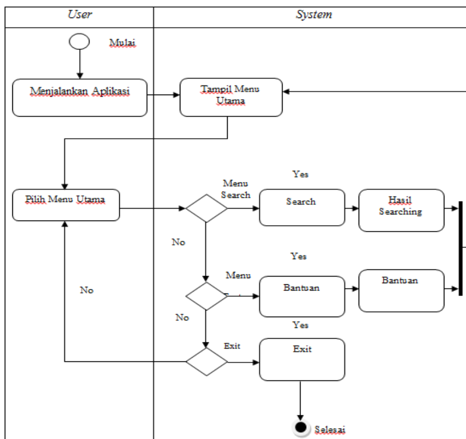
Gambar 2. Activity diagram
