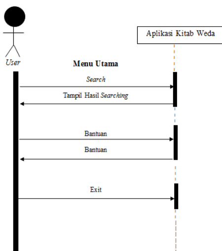
Gambar 3. Sequence diagram
