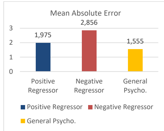
Figure 14. MAE for Regression Models
