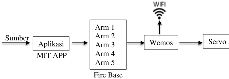
Gambar 1. Blok Diagram Arm Robot
