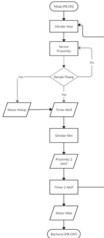
Gambar 2. Alur Program Arm Robot
