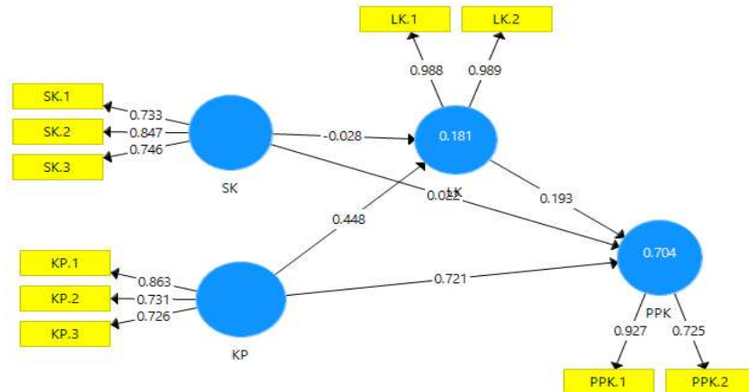
Gambar 2. Output Outer Loading CFA 2
