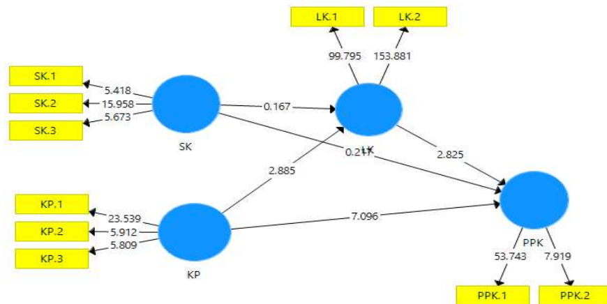
Gambar 3. Output Inner Model
