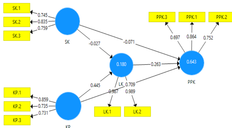
Gambar 1. Output Outer Loading CFA
