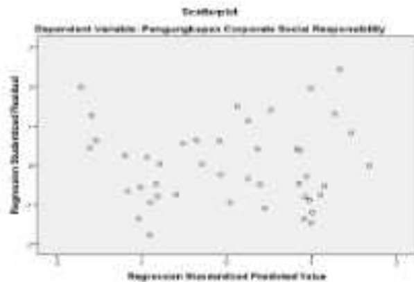
Gambar 2. Scatterplot
