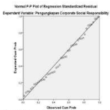
Gambar 1. Normal P-P Plot of Regression Standard Residual
