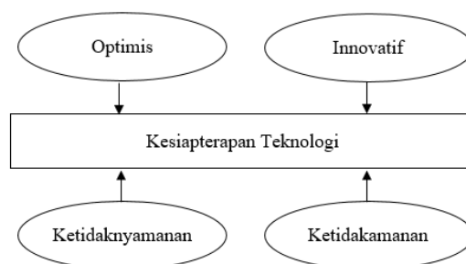
Gambar 2. Model Penelitian
