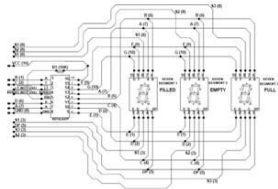
Gambar 5 Perancangan Typical Schematic drawing single seven segment
