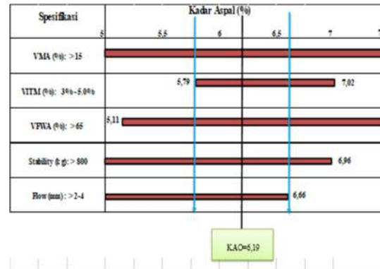
Fig 2. Optimum Asphalt Content graph
