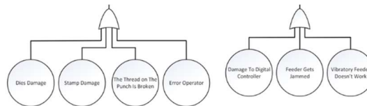
Figure 12. OR Gate and Basic Event
