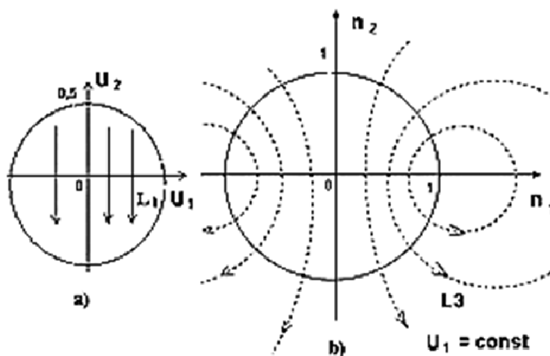
Figure 4. Correspondence of the plane U_1, U_2 , a): to conformal plane n_1, n_2 , b): for U_1 = \text{const}
