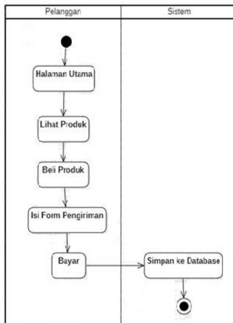
Gambar 7. Activity Diagram Order
