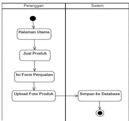
Gambar 6 Activity Diagram Jual
