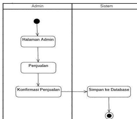
Gambar 8. Activity Diagram Validasi Penjualan
