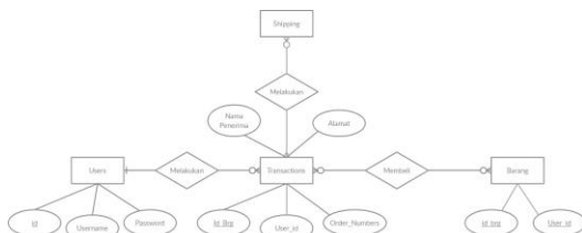
Gambar 10. ERD Database
