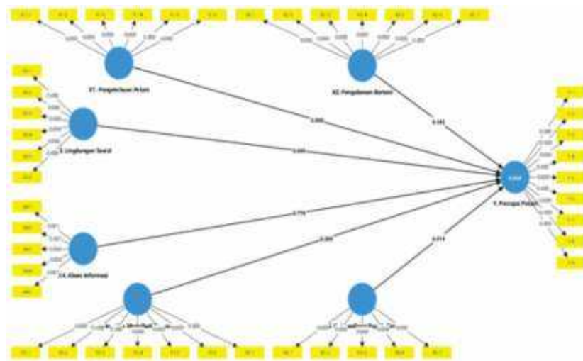
Gambar 2: Path Coefficients
