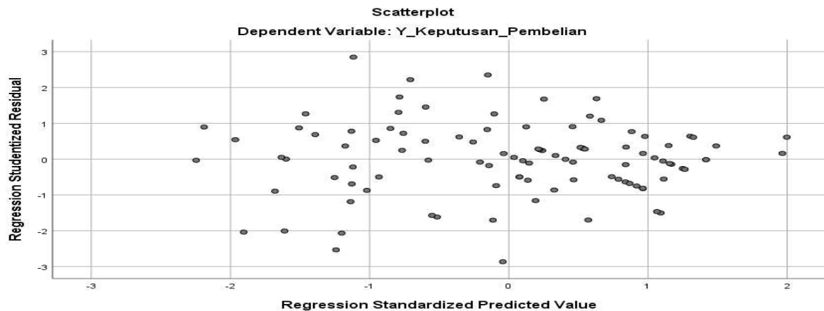
Figure 3. Scatterplot
