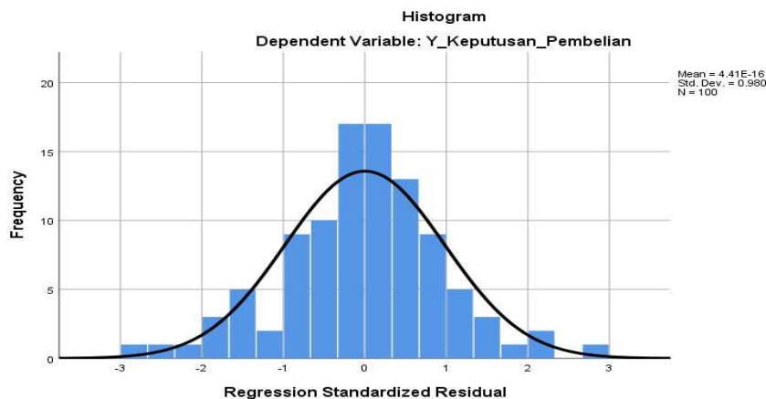
Figure 1. Histogram Graph
