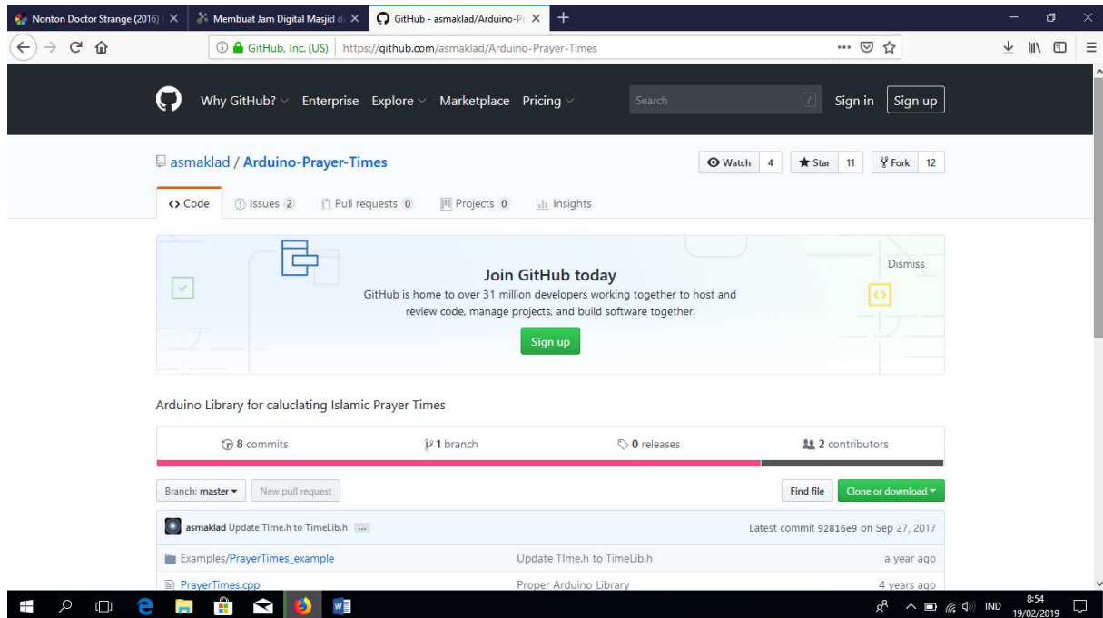
Gambar 2. Library PrayerTime
