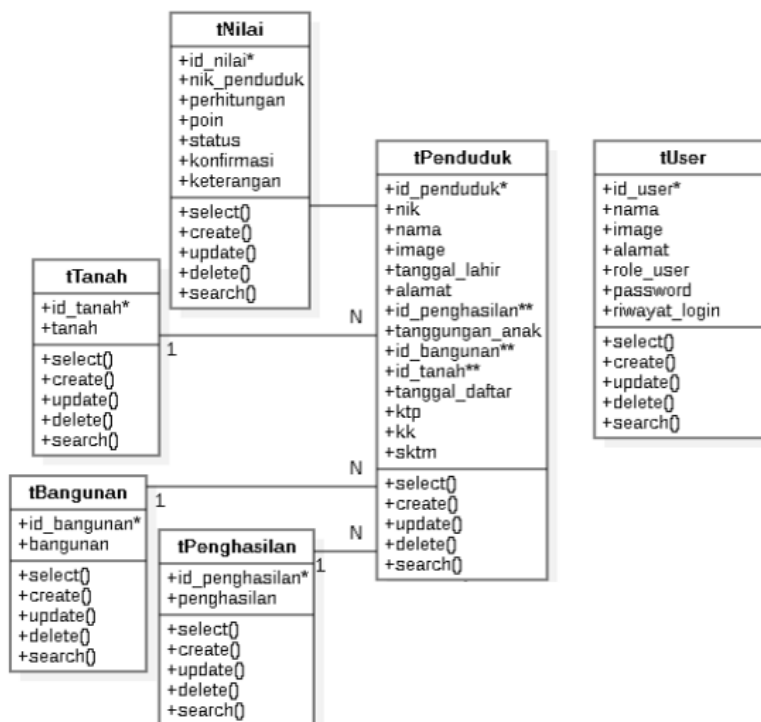
Gambar 4. Class Diagram
