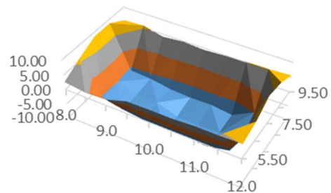
Gambar 10 Bending Momen 1 Lapis Matras
