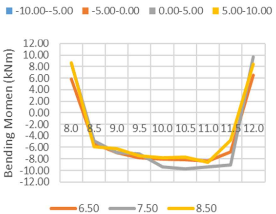
Gambar 11 Bending Momen 3 Lapis Matras
