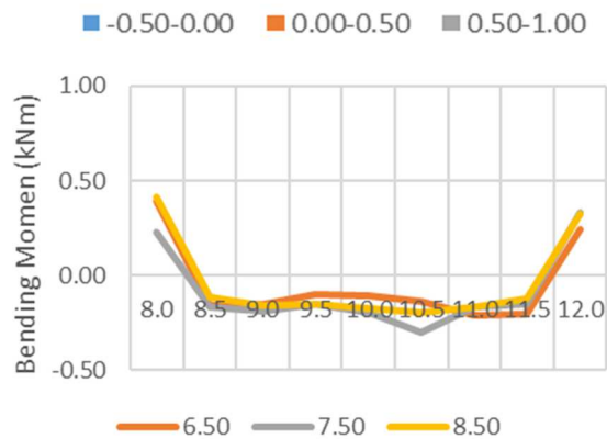
Gambar 10 Bending Momen 1 Lapis Matras
