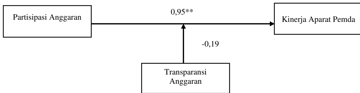
Gambar 2. Model Moderasi
