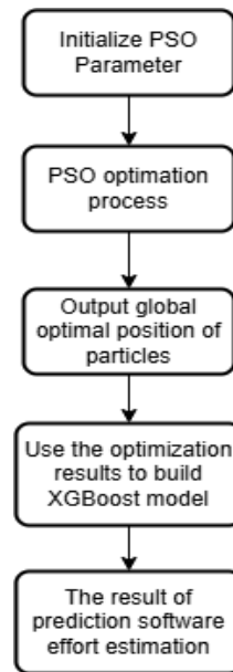
Gambar 1. PSO-XGBoost Process Flowchart
