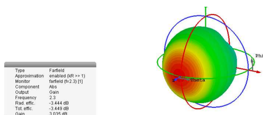
Gambar 7. Hasil simulasi gain antenna MIMO 2x2
