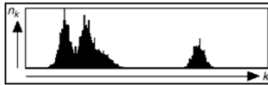
Gambar 1. Histogram Citra
