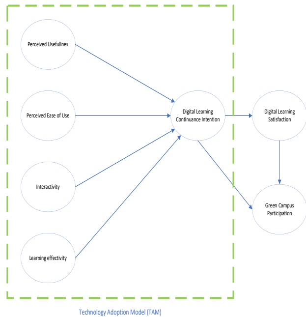
Gambar 2 Model penelitian
