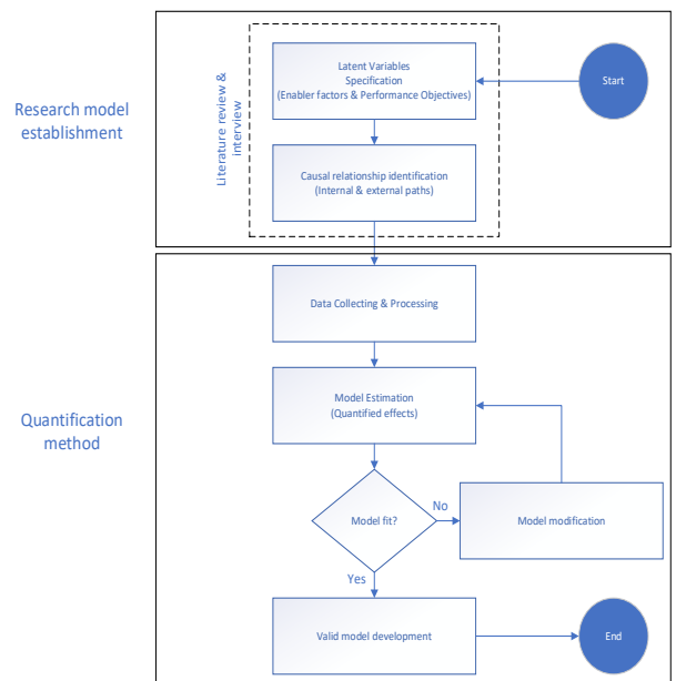
Gambar 3 Prosedur penelitian
