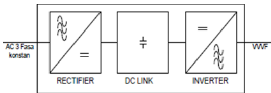
Gambar 3. Blok diagram variable speed drive 3 fasa
