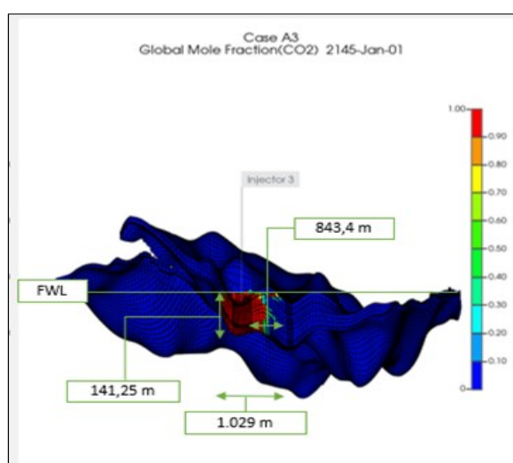
Figure 3. CO 2 plume geometry for well placement scenarios at 2145. (a) Case A1, (b) Case A2, and (c) Case A3 showing the spatial distribution of CO 2 mole fraction within the aquifer zone. The horizontal green line represents the free-water level (FWL), indicating the boundary between the aquifer and the overlying gas zone. Annotated values indicate key plume metrics, including lateral migration distance, plume width, and vertical plume rise relative to the injection point.
