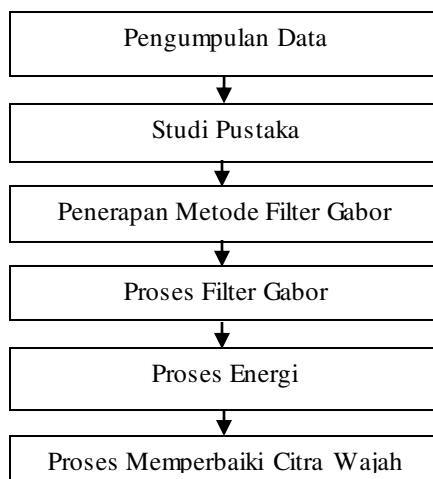
Gambar 1. Metode Penelitian
