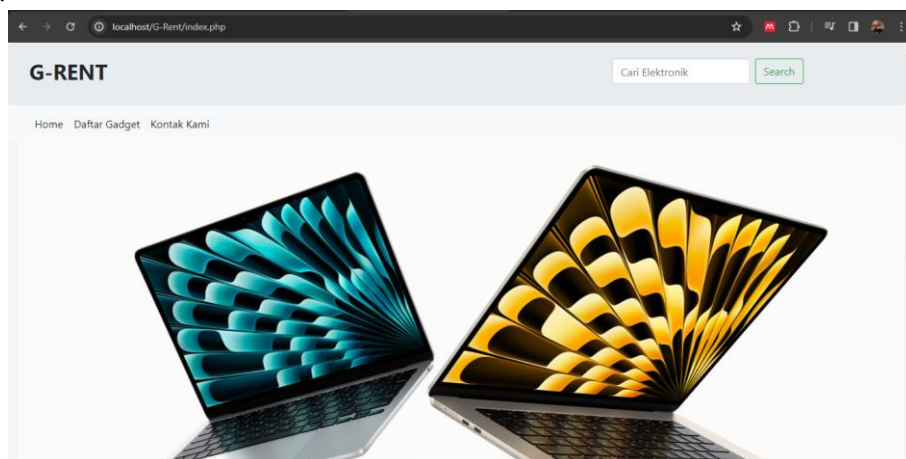
Gambar 1. 2 Halaman Home
