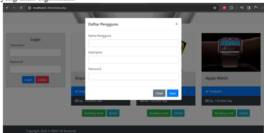
Gambar 1. 4 Halamn Register
