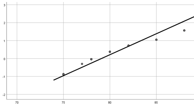
Picture 2. Normal Q-Q Plot of SMPN 1 Cisarua
