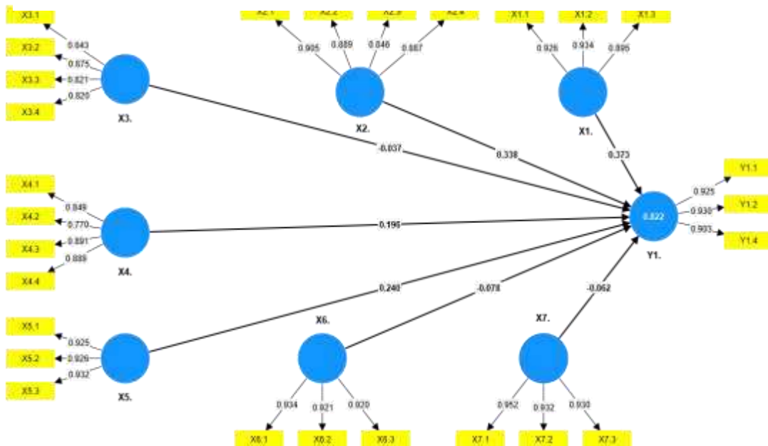
Gambar 1. Outer Loading
