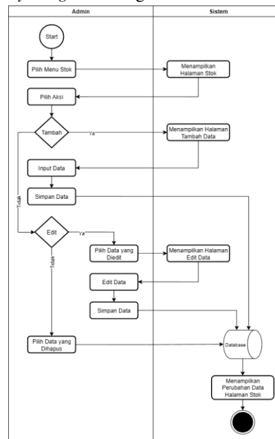
Gambar 2 Activity Diagram Mengelola Data Stok
