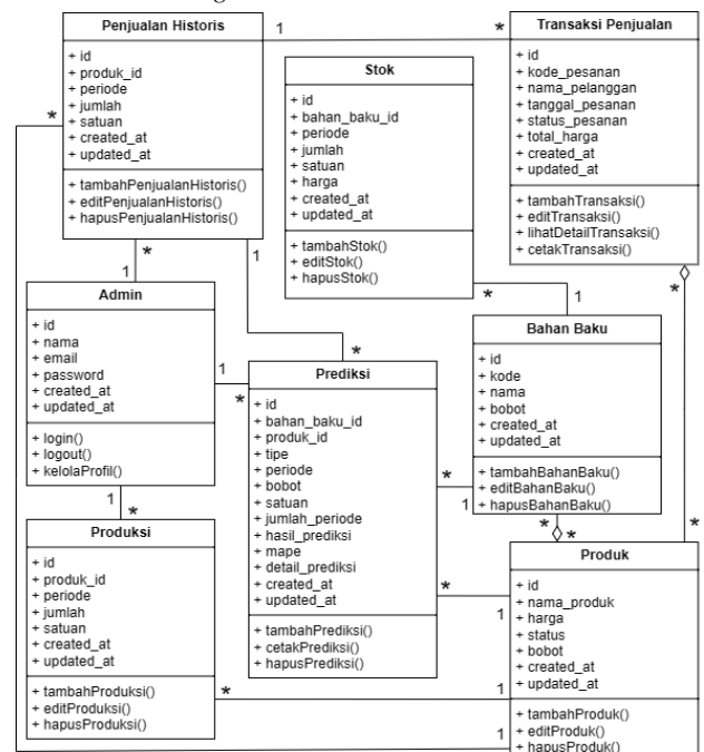
Gambar 6 Class Diagram
