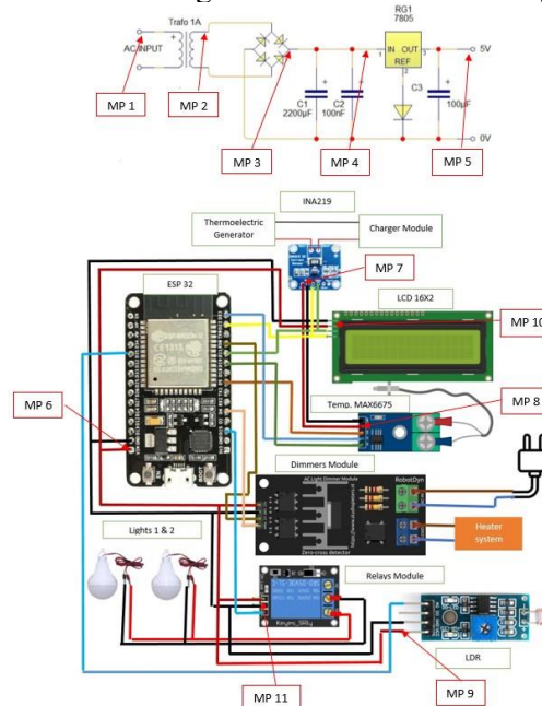
Figure 5. Tool Measurement Point
