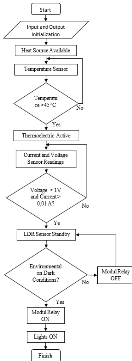
Figure 3. Flowchart system
