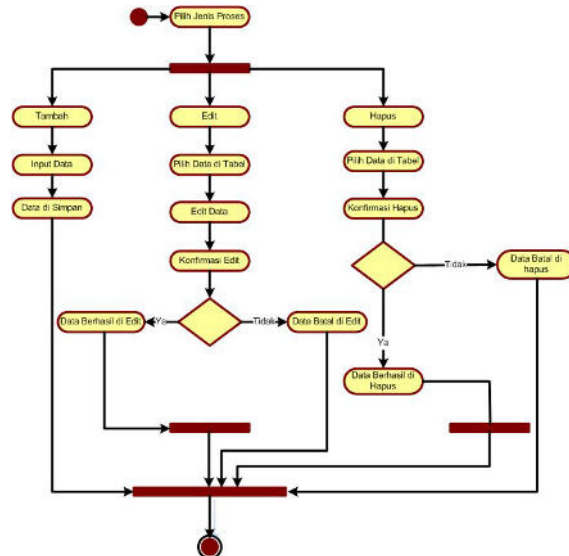
Gambar 4 Activity Diagram Proses Sistem
