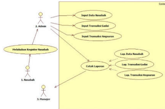
Gambar 1 Use Case
