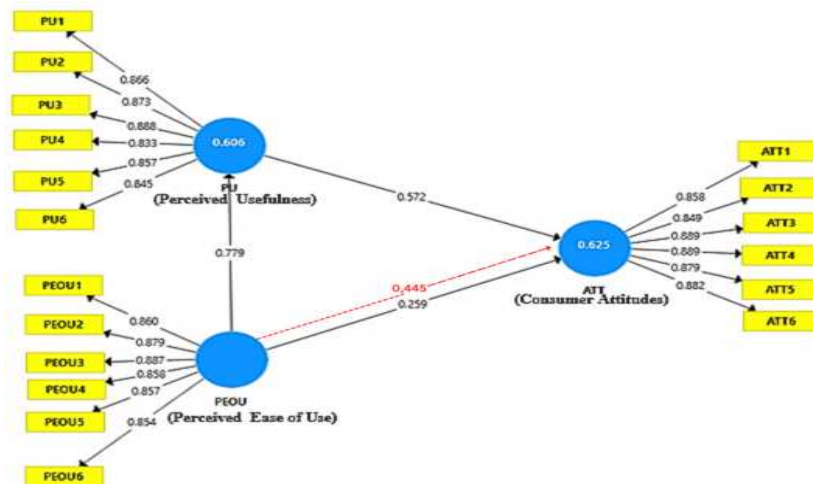
Gambar 3. Path Analysis
