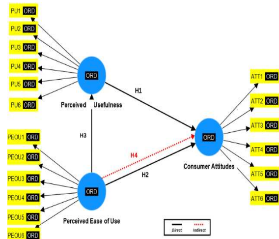
Gambar 2. Model Penelitian
