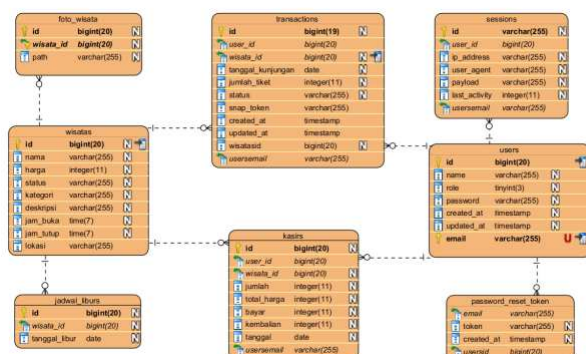
Figure 4. Entity Relationship Diagram
