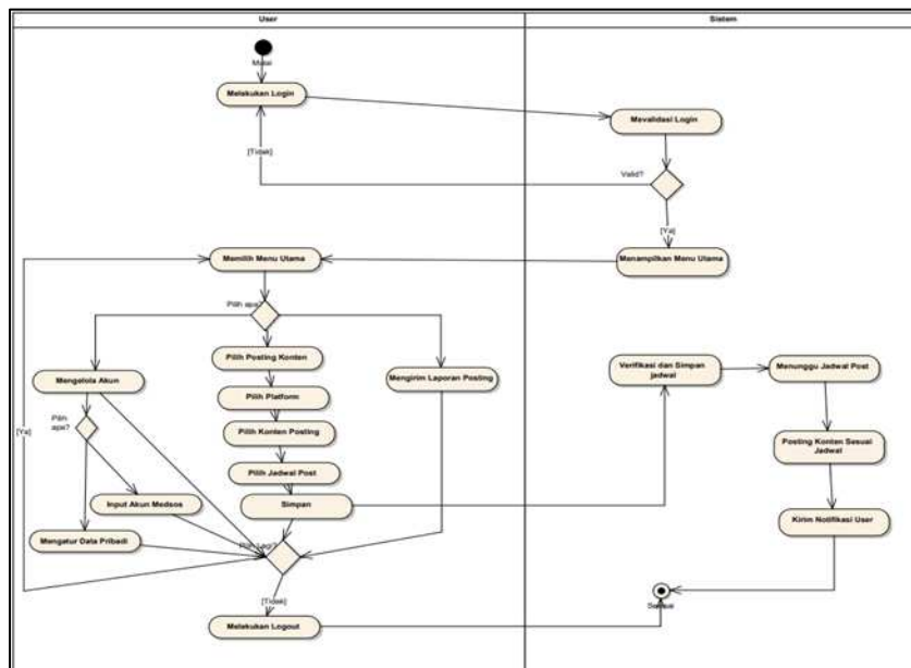
Gambar 3. Diagram Activity
