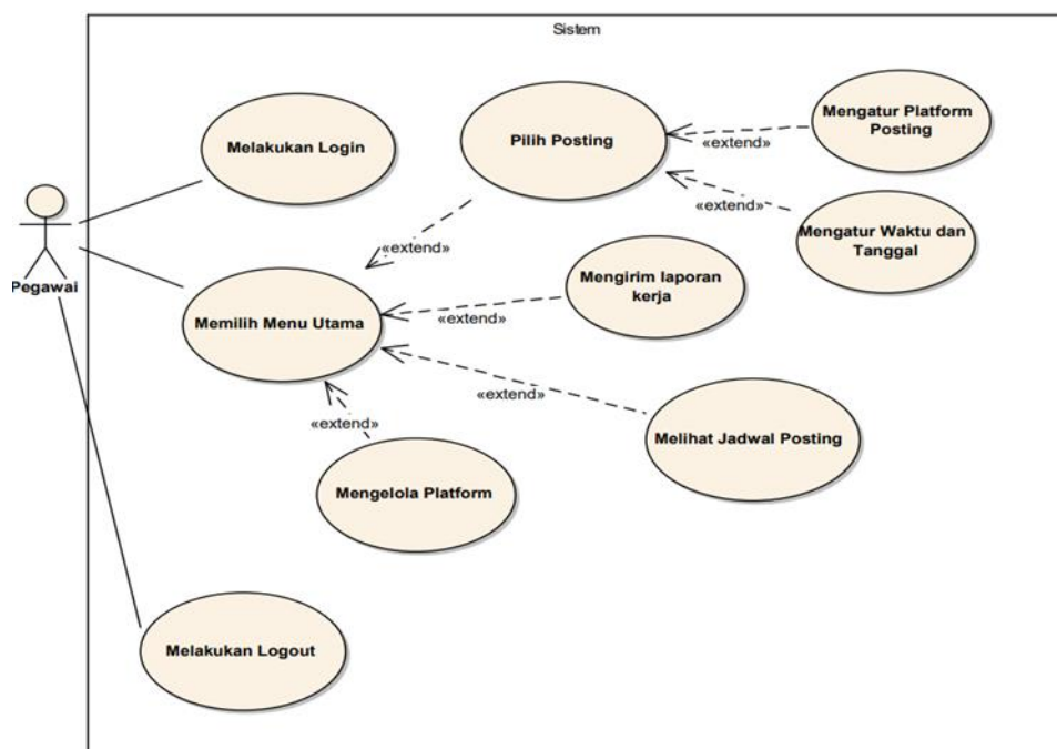
Gambar 2. Diagram Use Case
