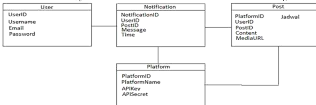
Gambar 4. Diagram Class
