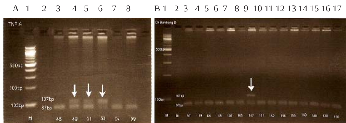
Figure 2. PCR results for TNF- \alpha 308G>A
