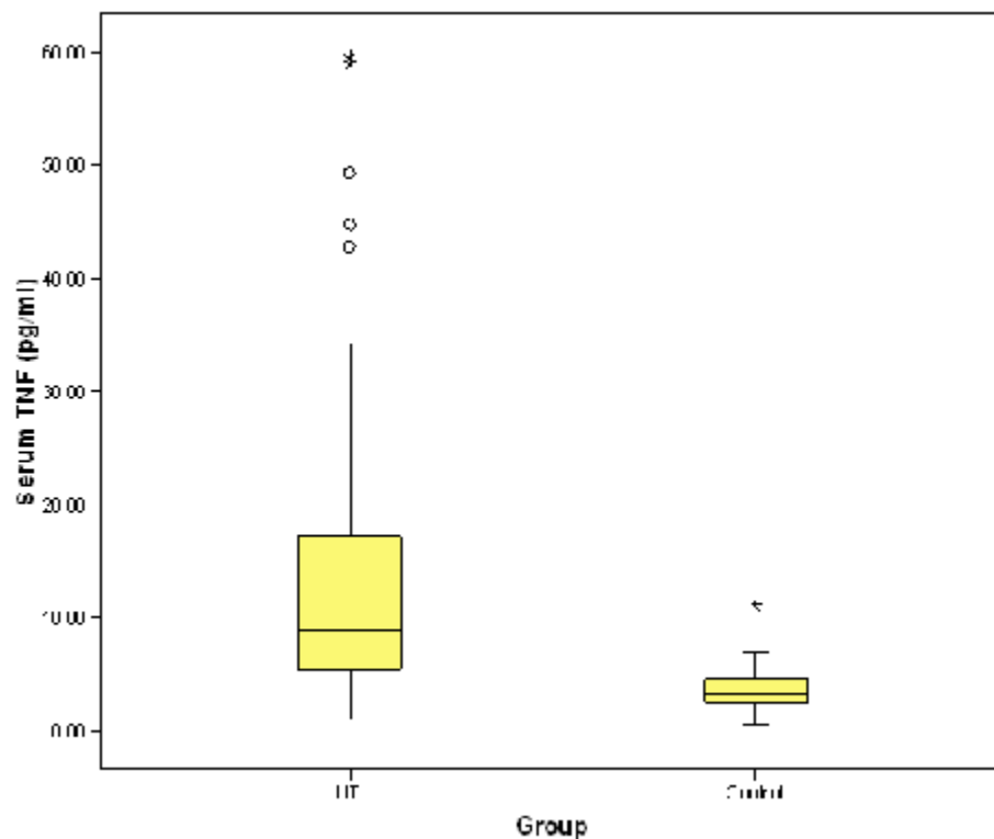
Figure 1. Box plots of TNF- \alpha serum levels. UTI due to E. coli (n=68); Non-UTI controls (n=55)
