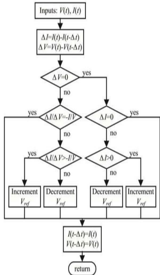
Gambar 4. Algoritma Incremental Conductance
