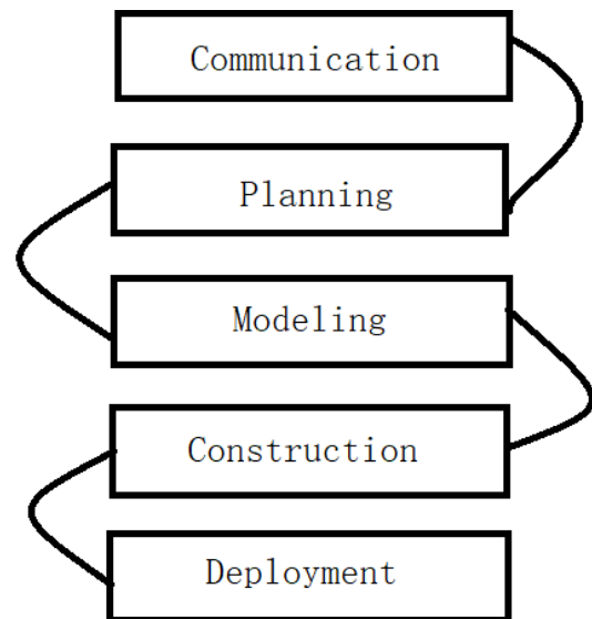
Gambar 1 Waterfall Model
