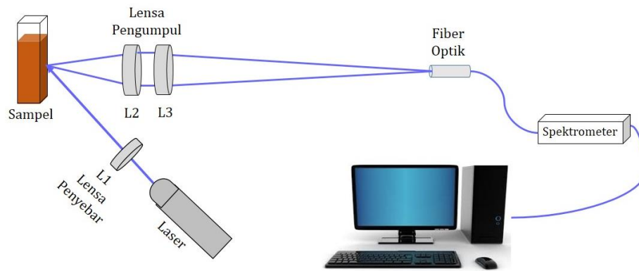
Gambar 2. Set up alat photoluminescence
