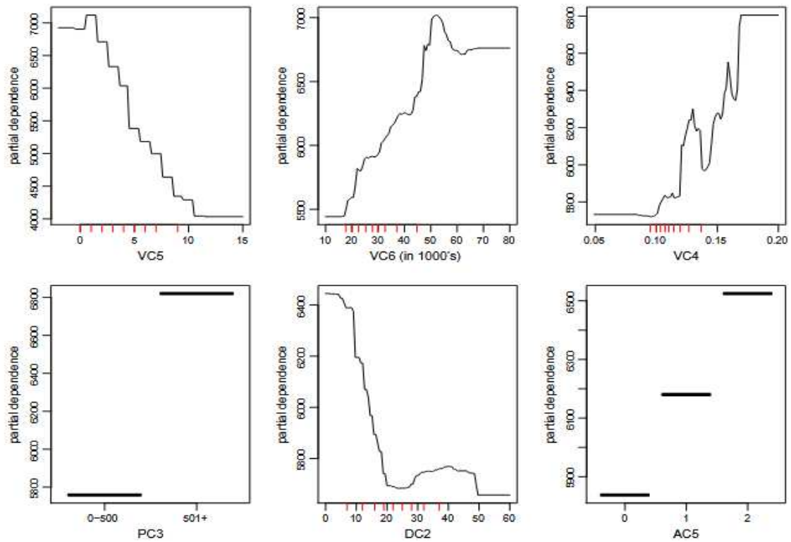
Gambar 7. Severity Model
