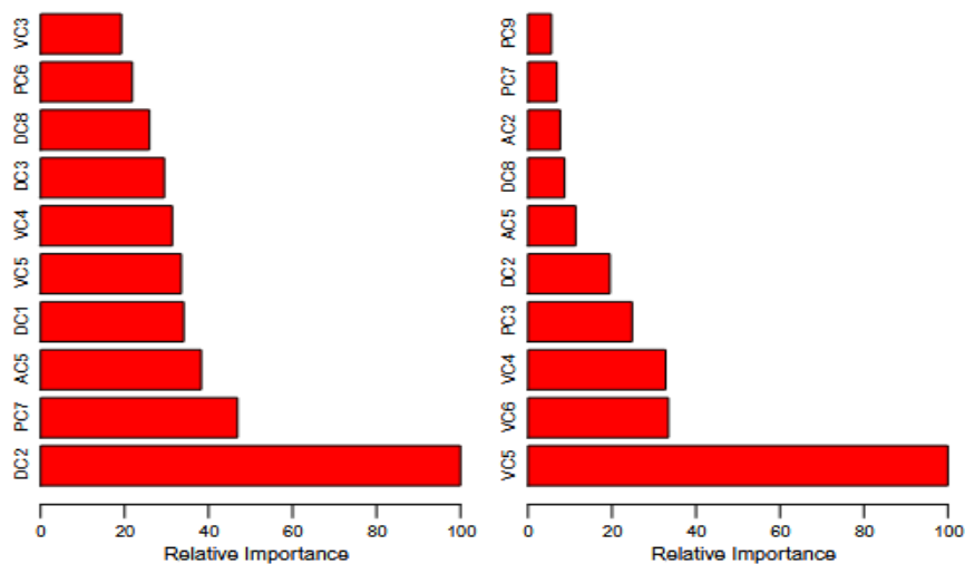
Gambar 5. Relative Importance
